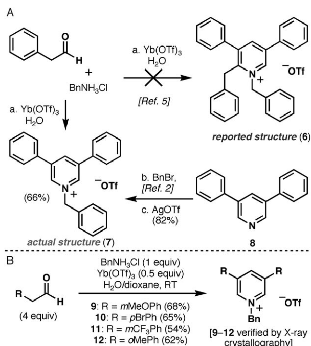
Scheme 1. Discovery of a mild “abnormal” Chichibabin pyridine synthesis. Reagents and conditions: a) phenylacetaldehyde (4.0 equiv), benzylammonium chloride (1.0 equiv), Yb(OTf) 3 (0.5 equiv), H 2 O, 23 °C, 66%; b) BnBr, acetone, 60 °C; c) AgOTf (1.1 equiv), CH 2 Cl 2 , 23 °C, 82% overall. Bn = benzyl, Tf = triflate.
