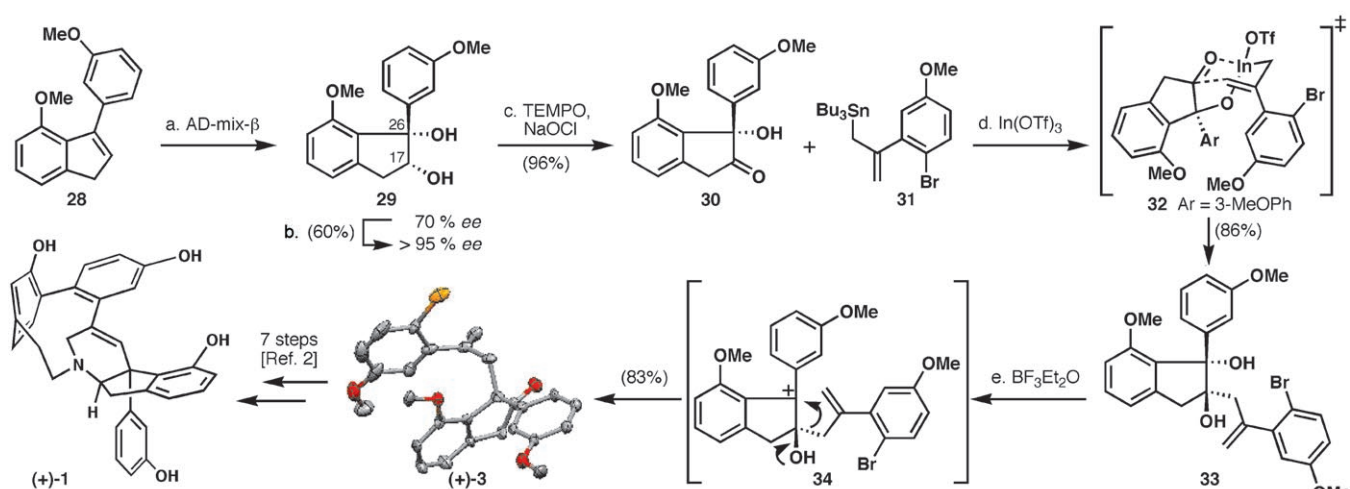
Scheme 4. Reagents and conditions: a) AD-mix- \beta , MeSO 2 NH 2 (5 equiv), 1:1 t BuOH/H 2 O, 5 °C, 44 h; b) crystallization, 60% overall; c) TEMPO (0.05 equiv), NaOCl (2.0 equiv), CH 2 Cl 2 /sat. aq NaHCO 3 (2.6:1), 0 °C, 30 min, 96%; d) 31 (2.0 equiv), In(OTf) 3 (1.2 equiv), THF, 0–23 °C, 86%; e) BF 3 Et 2 O (1.1 equiv), CH 2 Cl 2 , 0 °C, 10 min, 83%. TEMPO = 2,2,6,6-tetramethylpiperidinyl-1-oxyl.
