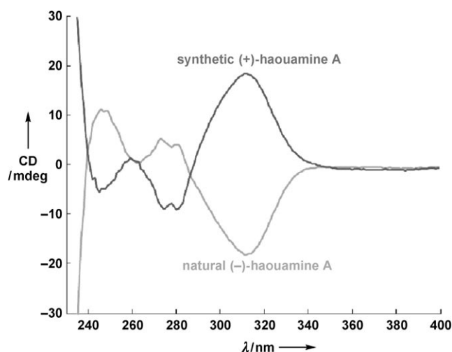
Figure 2. Circular dichroism spectrum.
